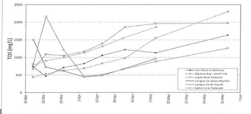
Last Mountain Lake Tributary Water Quality – 2015
