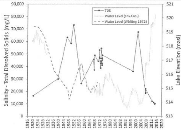
Figure 1: Historic salinity and water level data for Big Quill Lake. Salinity data are from sources cited in the text and from Garth van der Kamp (pers. comm.). Water level data is from the Water Survey of Canada (Environment Canada) and Whiting (1972). Environment Canada water level data prior to 1932 were estimated by the Saskatchewan Water Security Agency based on historic elevation data and a re-established benchmark.
