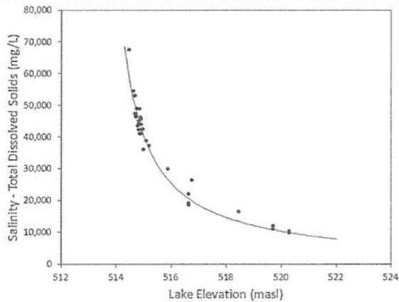
Figure 2: Relationship between salinity and lake elevation for Big Quill Lake. Water level data on water quality sampling dates were interpolated between adjacent dates. Salinity data sources are the same as Figure 1, except winter and spring values (from Hammer 1973) were removed from the dataset as were those between 1931 and 1956 because of the paucity of water level data. Winter and spring data were removed because the principal interest was to establish a relationship between typical salinity and lake level, which can be biased during winter because of brine rejection during surface ice formation and biased during spring if the separation of inflowing water and/or vertical differences in lake salinity still persists from winter. Curve Expert (version 1.38) was used to find the line of best fit, which was a saturation growth-rate model ( \text{salinity} = (131.96 \times \text{lake elevation}) / (-513.30968 + \text{lake elevation}) ; r^2 = 0.96 ). This line is extrapolated beyond the high elevation data to provide a rough initial estimate of salinity if Big Quill Lake continues to increase in elevation.
