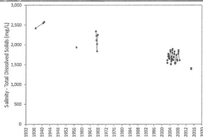
Figure 6: Last Mountain Lake salinity (total dissolved solids).
