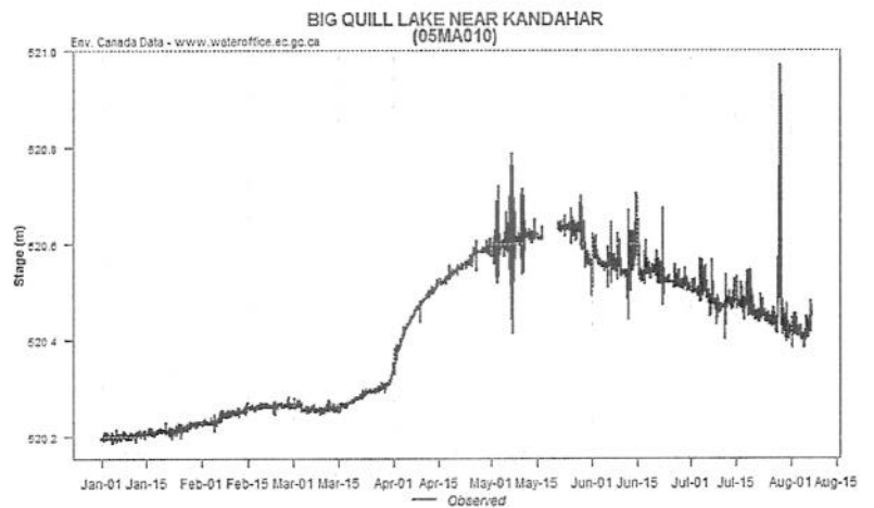
Big Quill Lake 2015 Hydrograph
